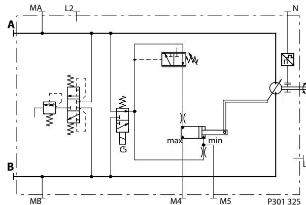
Hydraulic schematic
