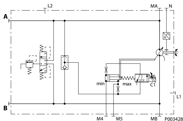
Hydraulic schematic
