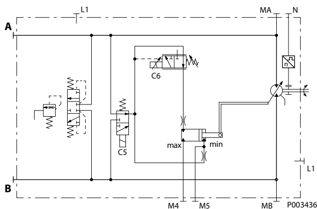
Hydraulic schematic
