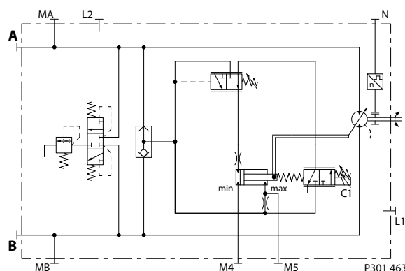
Hydraulic schematic
