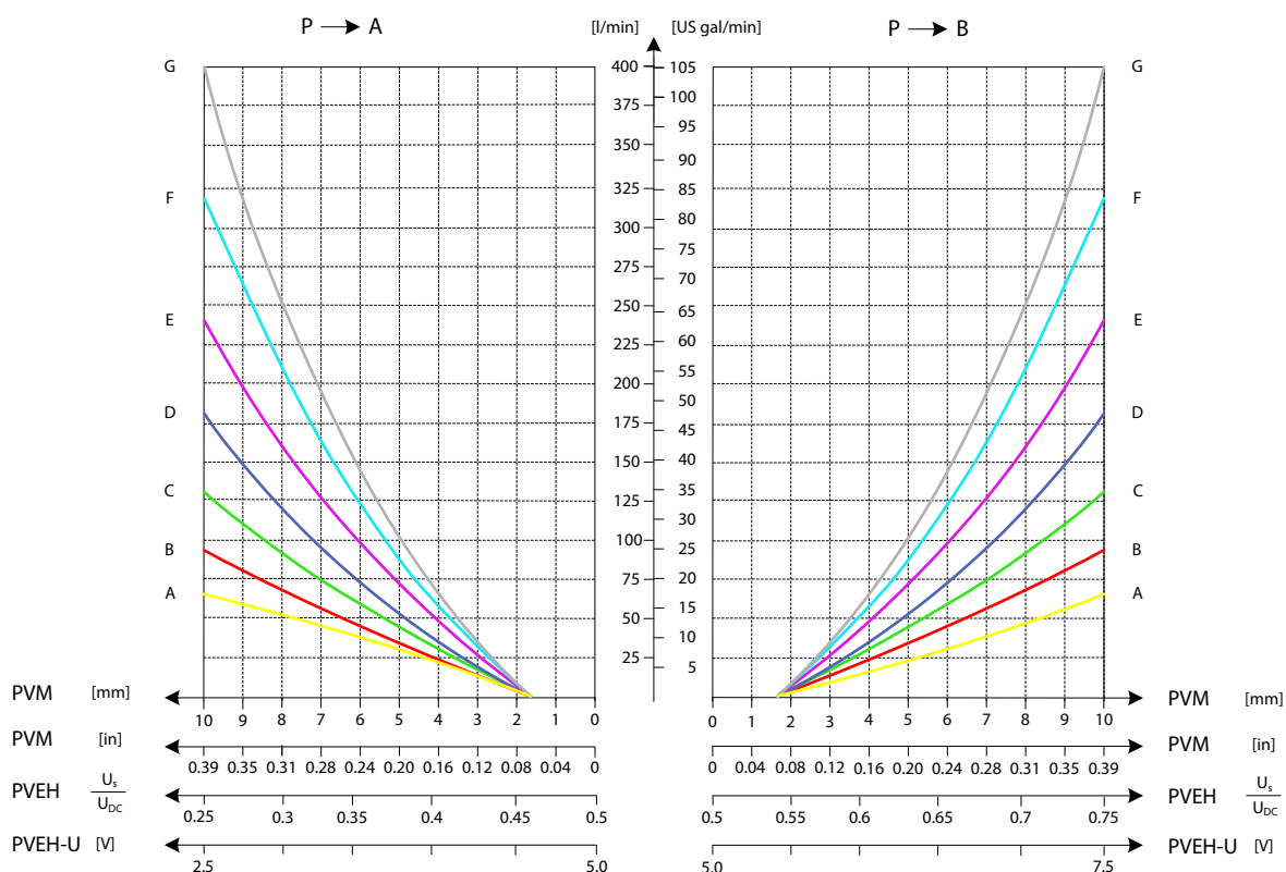
Oil Flow as Function of Spool Travel
