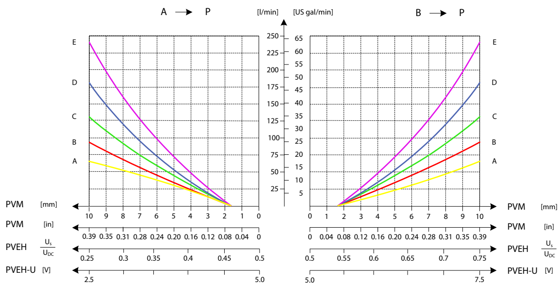
Oil flow as function of spool travel
