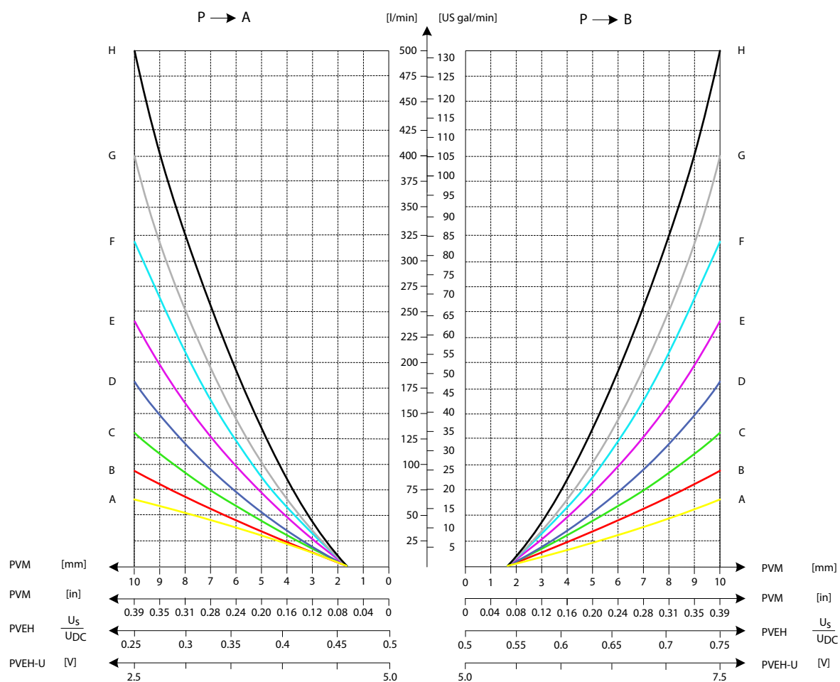
Oil Flow as Function of Spool Travel
