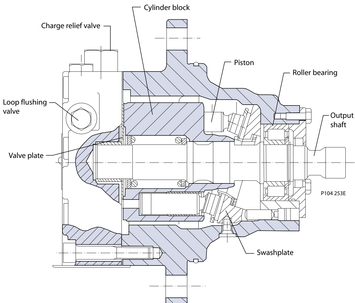
Cross section
