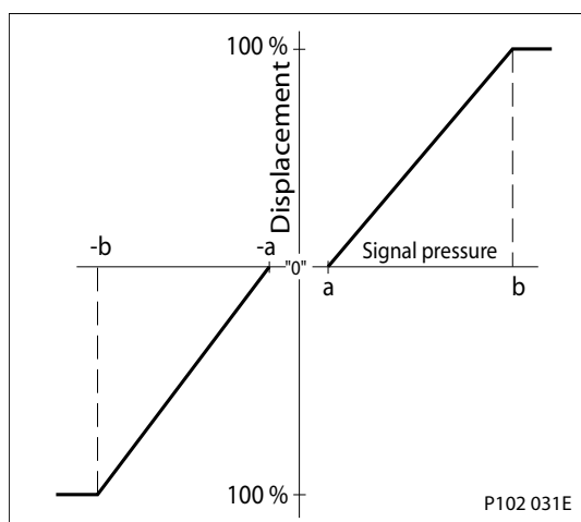
Pump displacement vs. signal pressure
