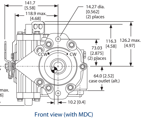
Front view (with MDC)
