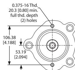
Rear view (no pads shown)
